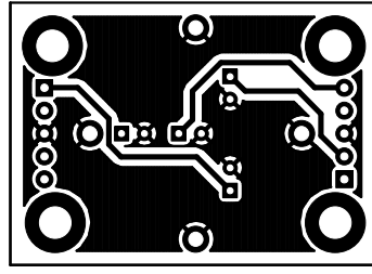
TOP ROUTING
