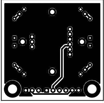
TOP ROUTING
