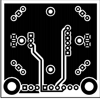
BOTTOM ROUTING
